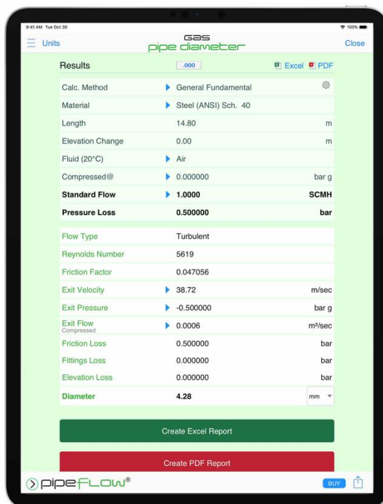
Figure 30 Gas Pipe Diameter Results
